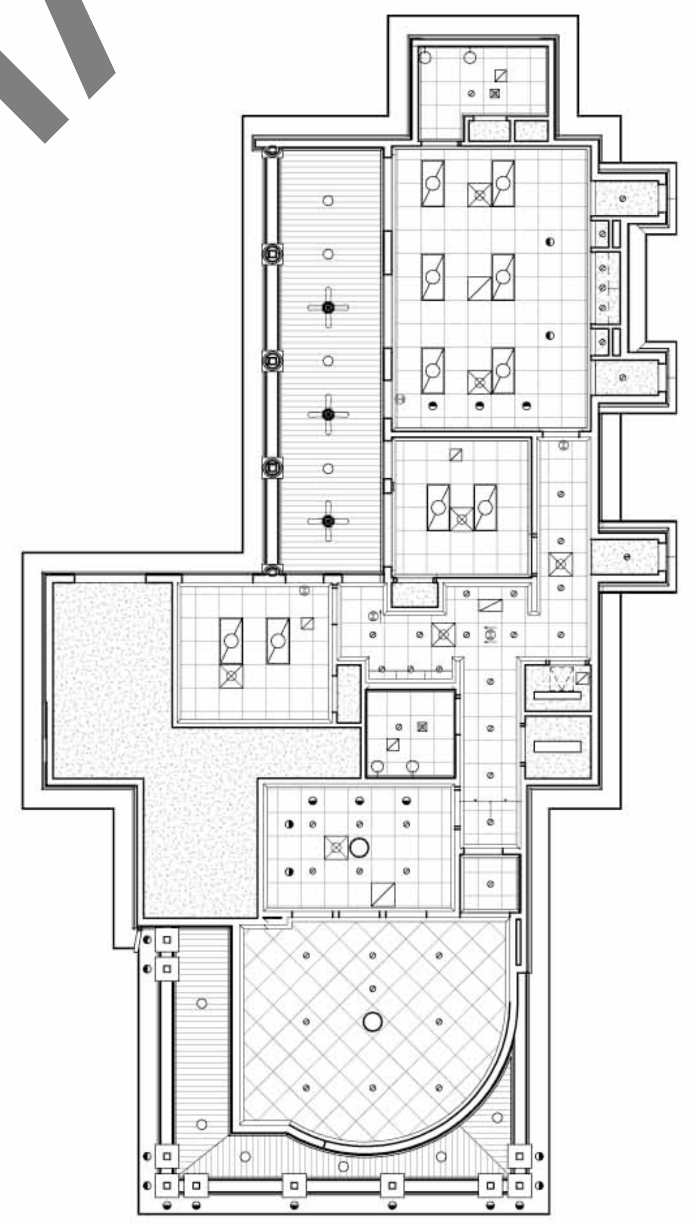
0.8 2nd FLOOR REFLECTED CEILING PLAN SCALE= 1/8" = 1'-0"
