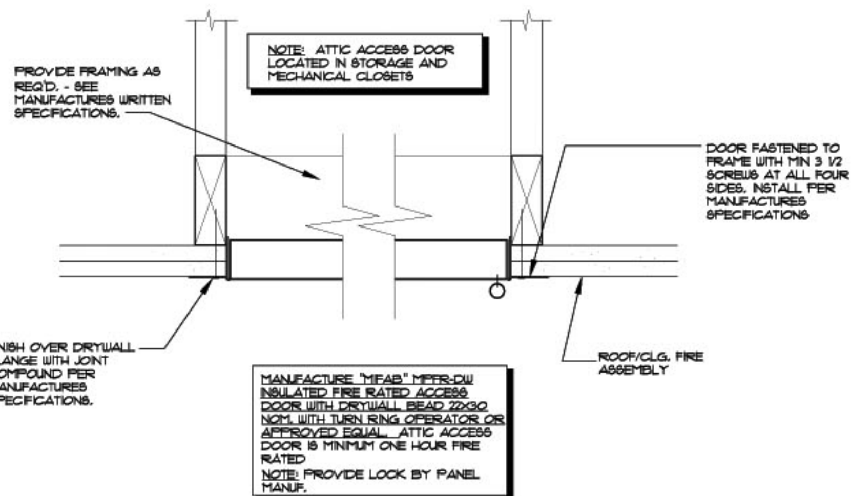
03 ATTIC ACCESS HATCH DETAIL 1 1/2" = 1'-0"
