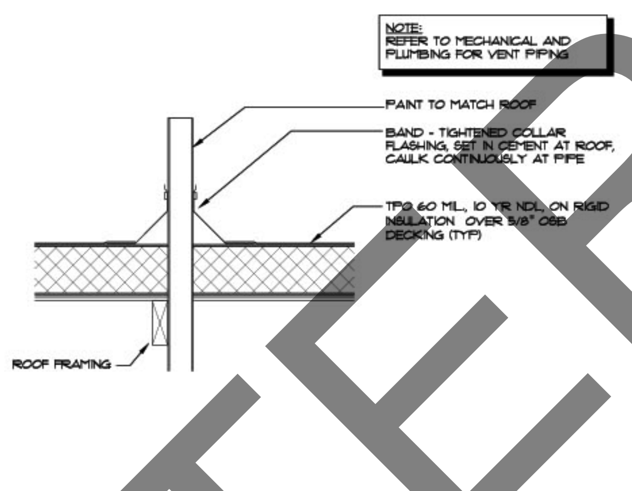
02 ROOF VENT DETAIL 1 1/2" = 1'-0"
