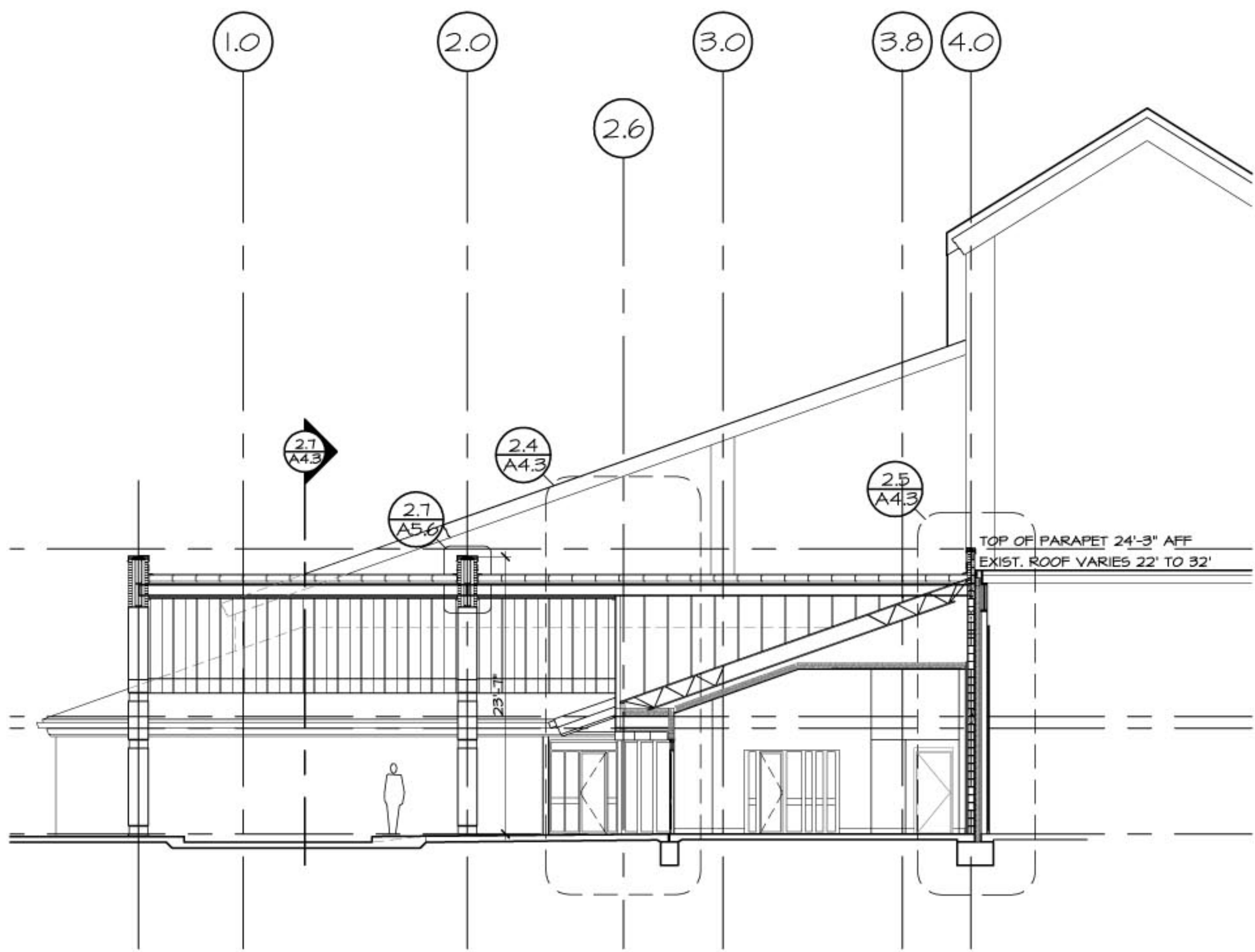
2.4 BLDG SECTION @ ENTRY SCALE: 1/8" = 1'-0"
