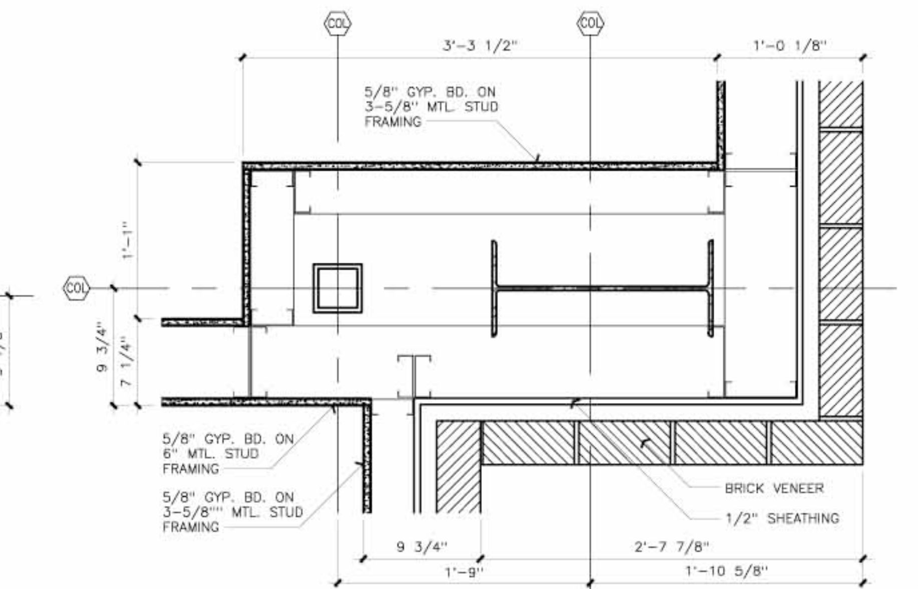
13 Column Detail SCALE 1 1/2"=1'-0"
