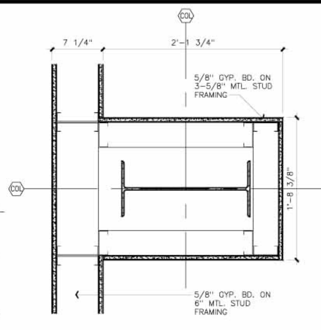
03 Column Detail SCALE 1 1/2"=1'-0"
