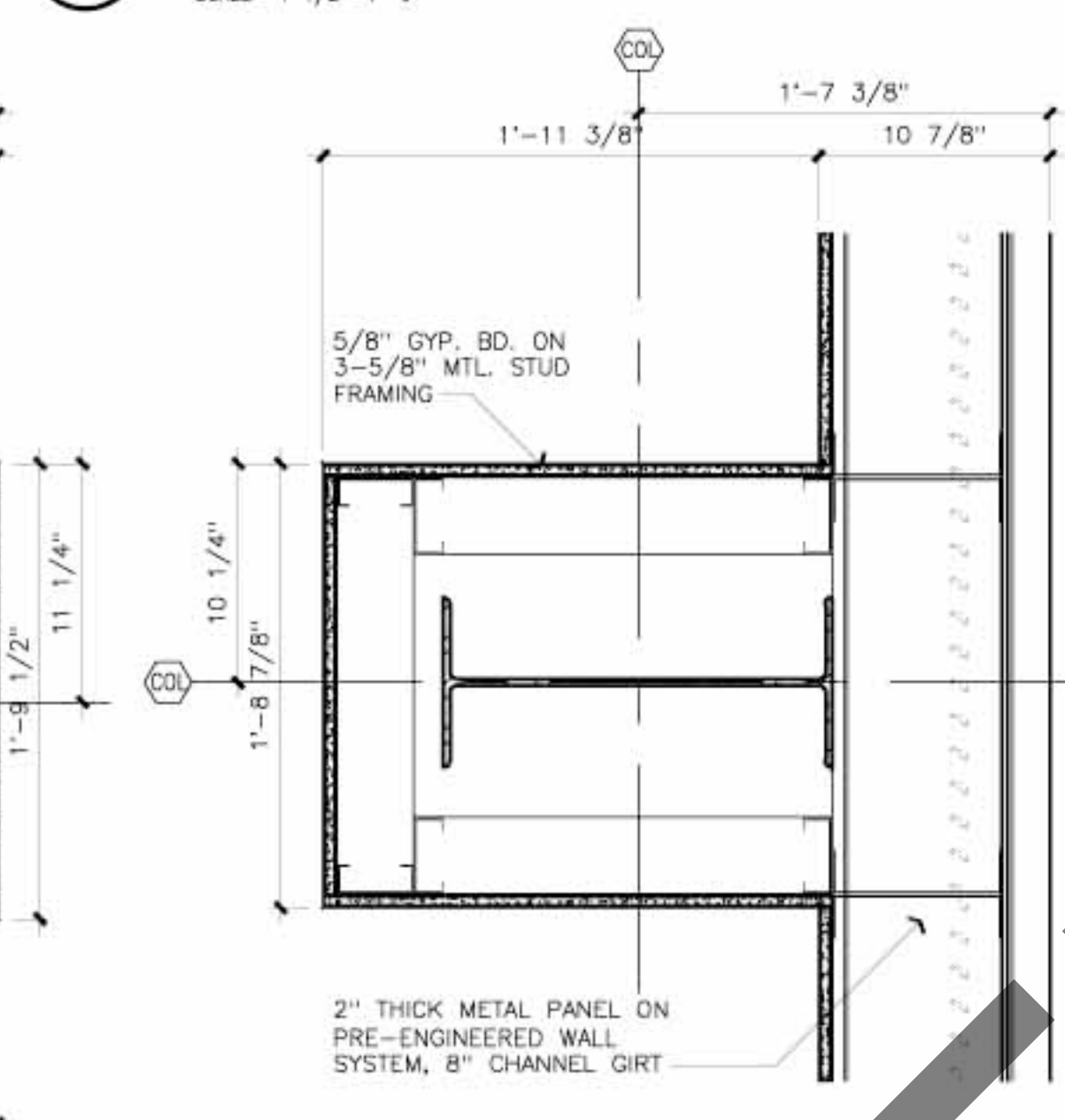
07 Column Detail SCALE 1 1/2"=1'-0"
