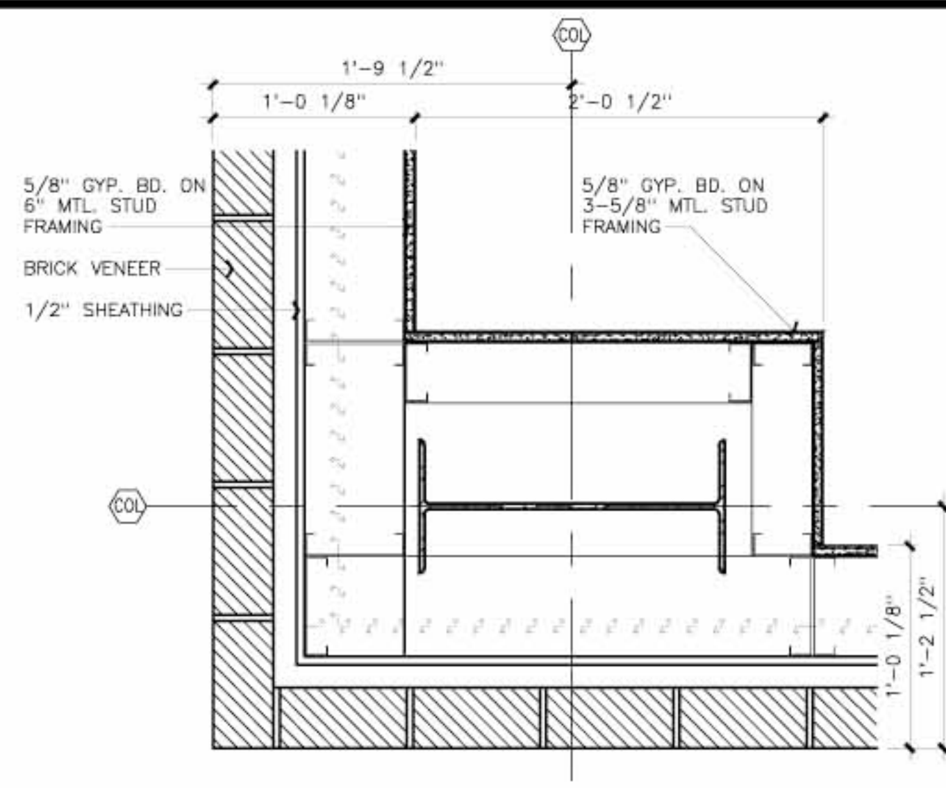
02 Column Detail SCALE 1 1/2"=1'-0"
