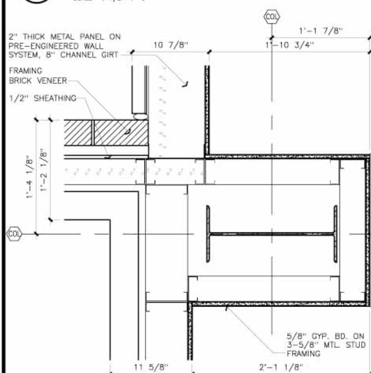
06 Column Detail SCALE 1 1/2"=1'-0"
