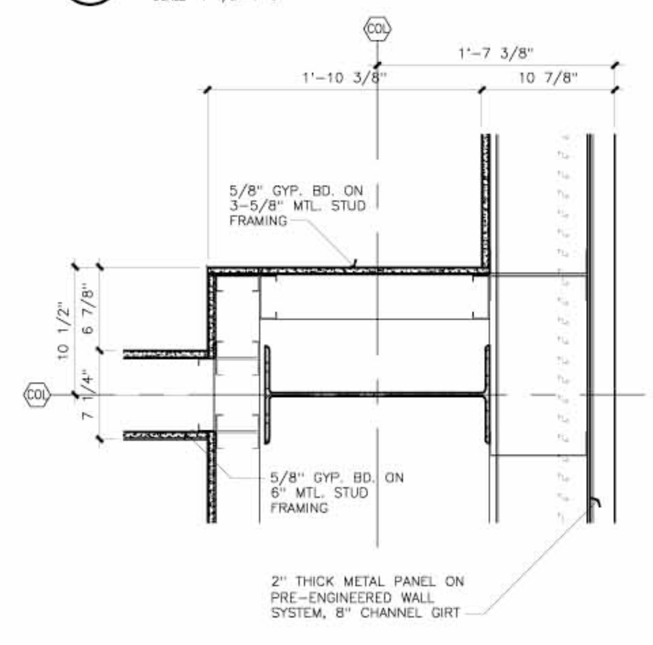
09 Column Detail SCALE 1 1/2"=1'-0"
