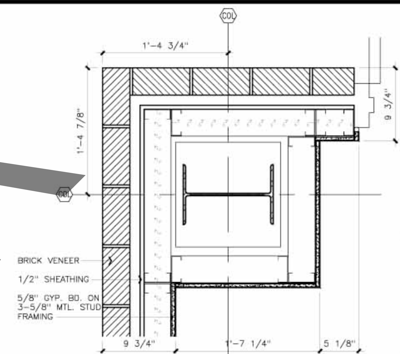
05 Column Detail SCALE 1 1/2"=1'-0"
