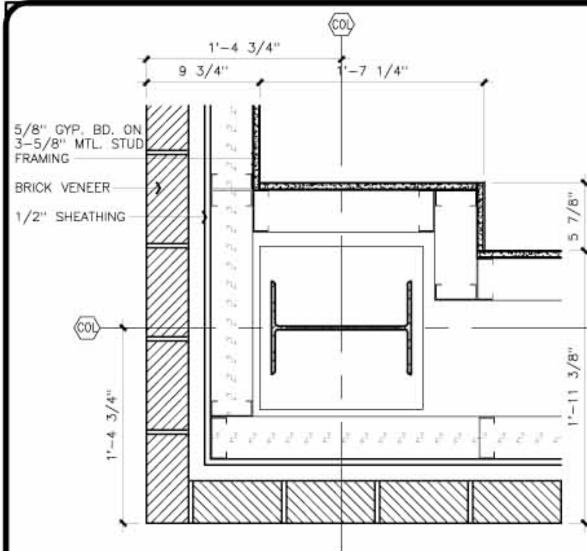
01 Column Detail SCALE 1 1/2"=1'-0"
