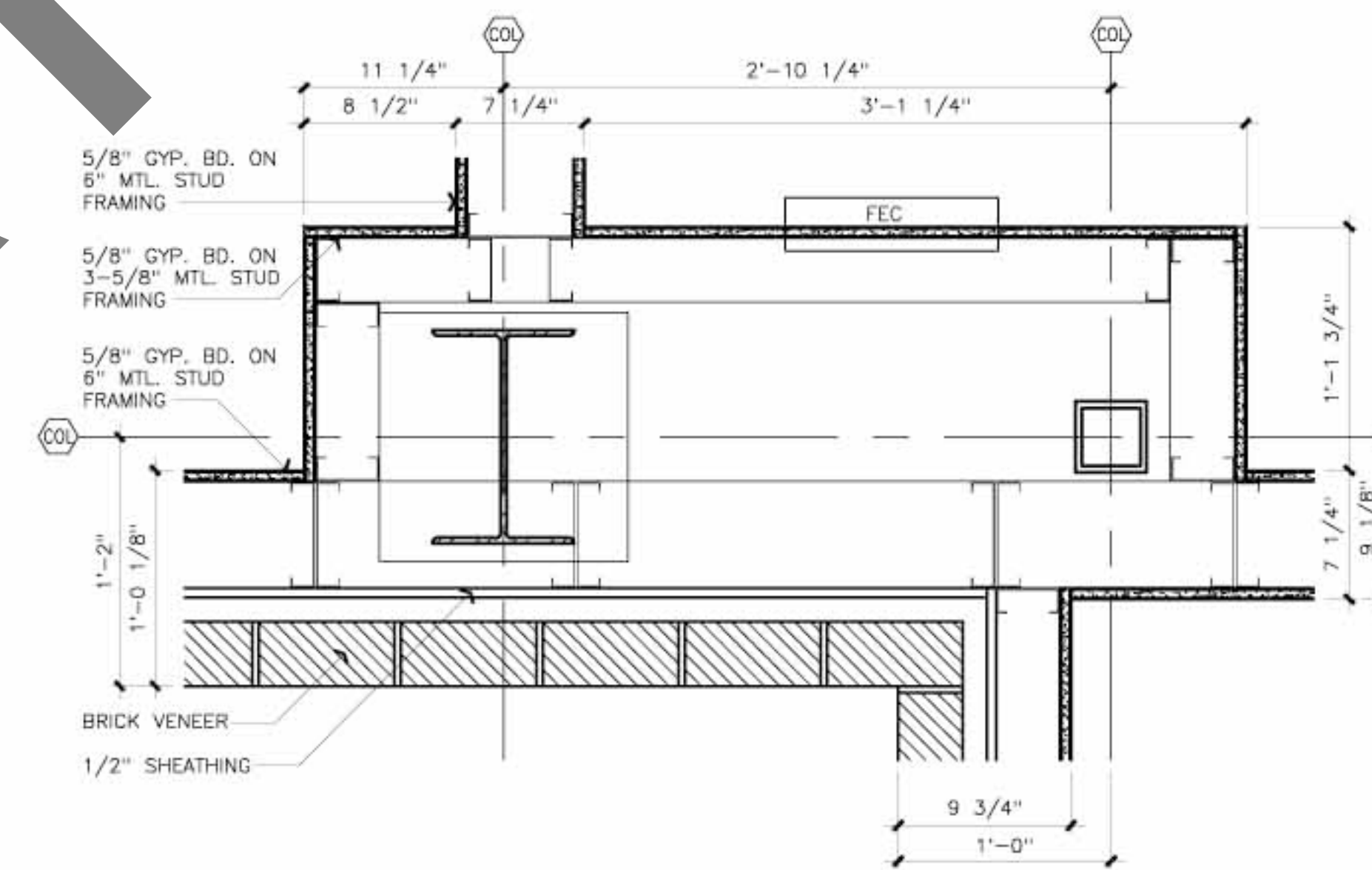
12 Column Detail SCALE 1 1/2"=1'-0"
