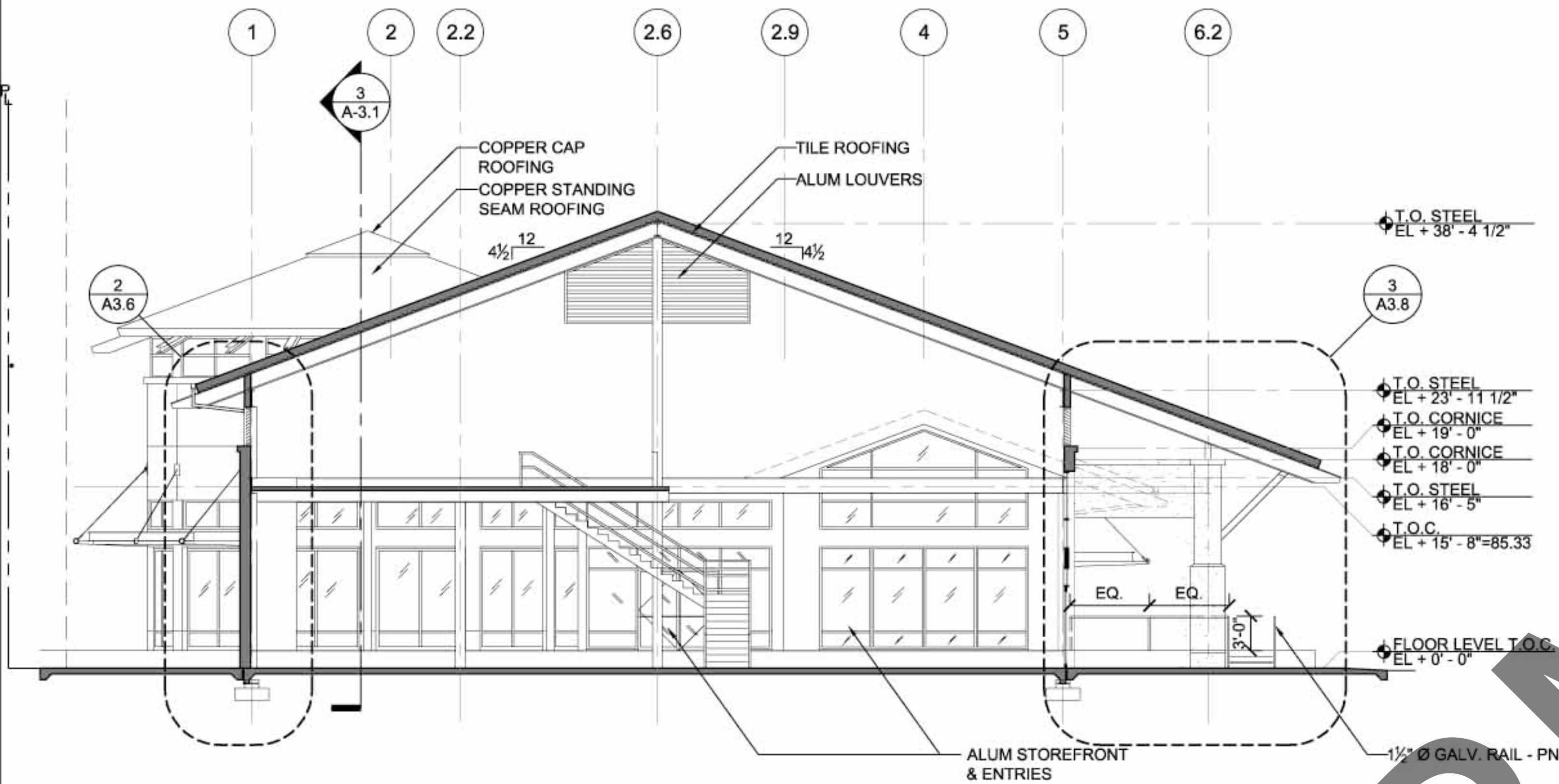
1 NF BUILDING SECTION SCALE: 1/8" = 1'-0"
