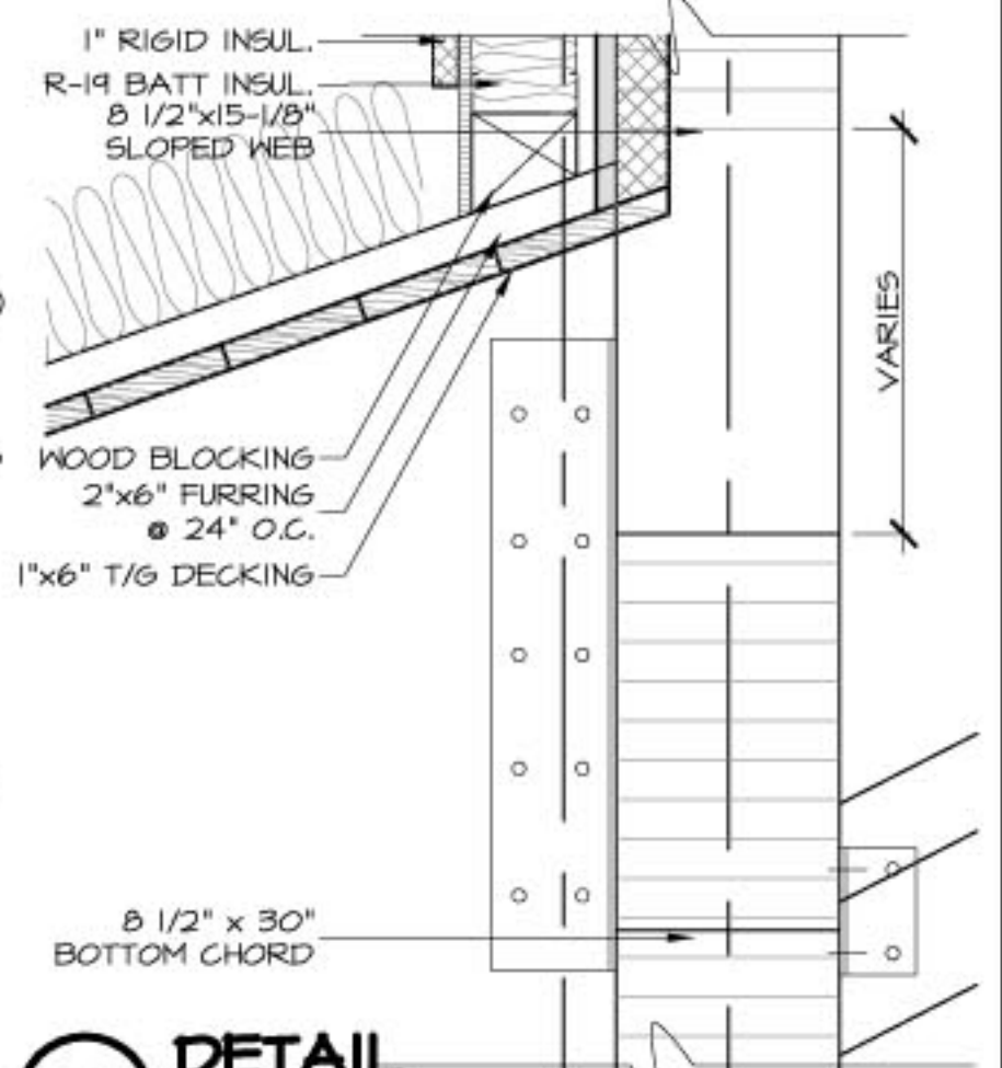
0.9 DETAIL SCALE: 1/2" = 1'-0"
