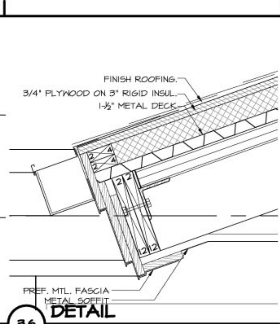
3.5 DETAIL SCALE: 1/2" = 1'-0"
