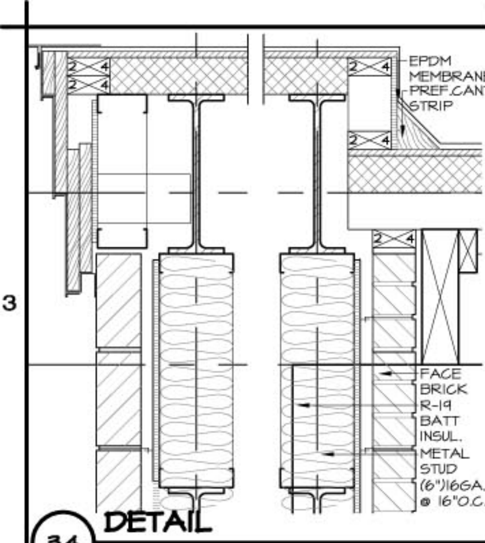
3.5 DETAIL SCALE: 1/2" = 1'-0"
