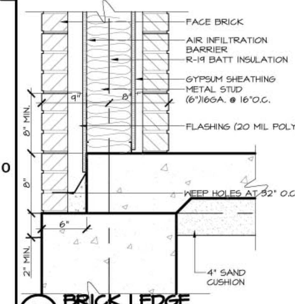
0.4 BRICK LEDGE SCALE: 1/2" = 1'-0"
