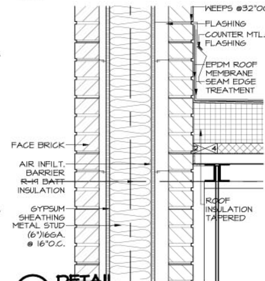
2.5 DETAIL SCALE: 1/2" = 1'-0"
