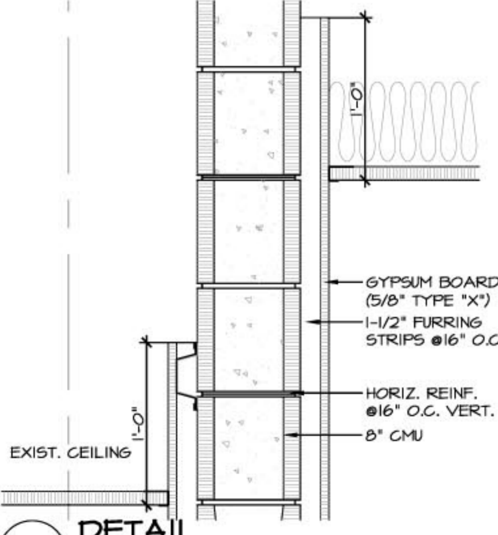
0.4 DETAIL SCALE: 1/2" = 1'-0"
