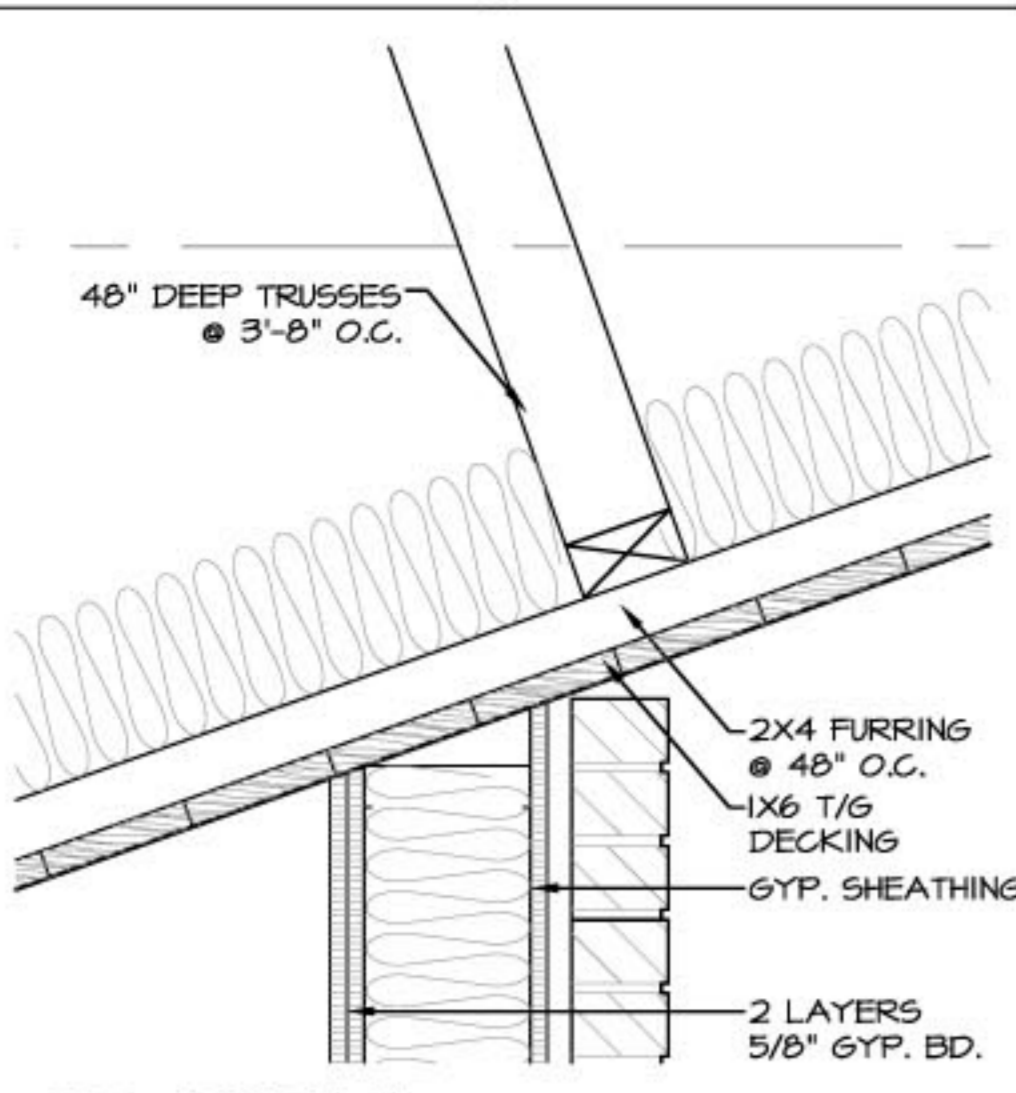
3.5 DETAIL SCALE: 1/2" = 1'-0"
