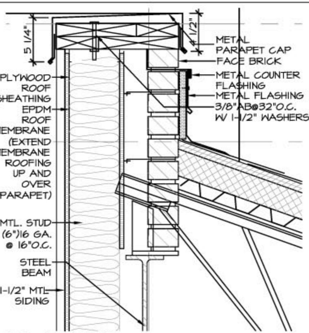
3.7 DETAIL SCALE: 1/2" = 1'-0"
