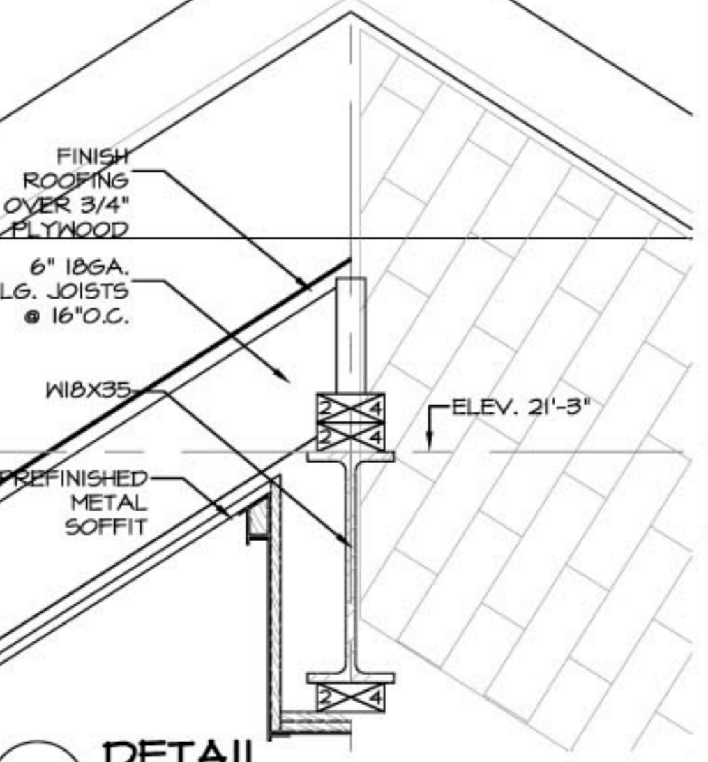
0.9 DETAIL SCALE: 1/2" = 1'-0"
