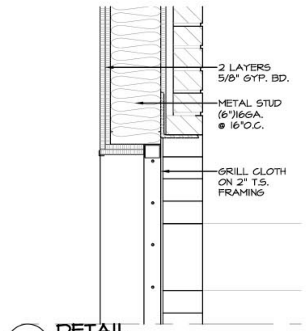
2.5 DETAIL SCALE: 1/2" = 1'-0"
