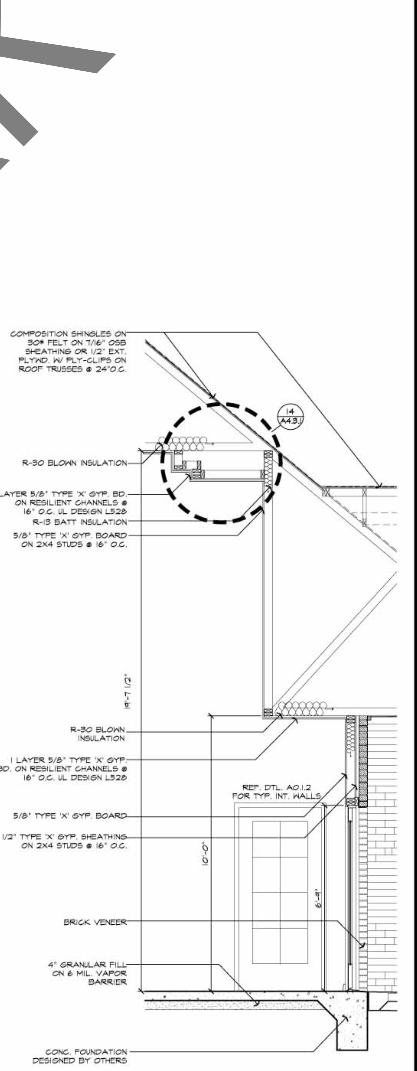
④ WALL SECTION @ COMMUNITY BLDG. 1/2" = 1' - 0" (A2.1.5) (1/A2.2.5) (A2.4.5)
