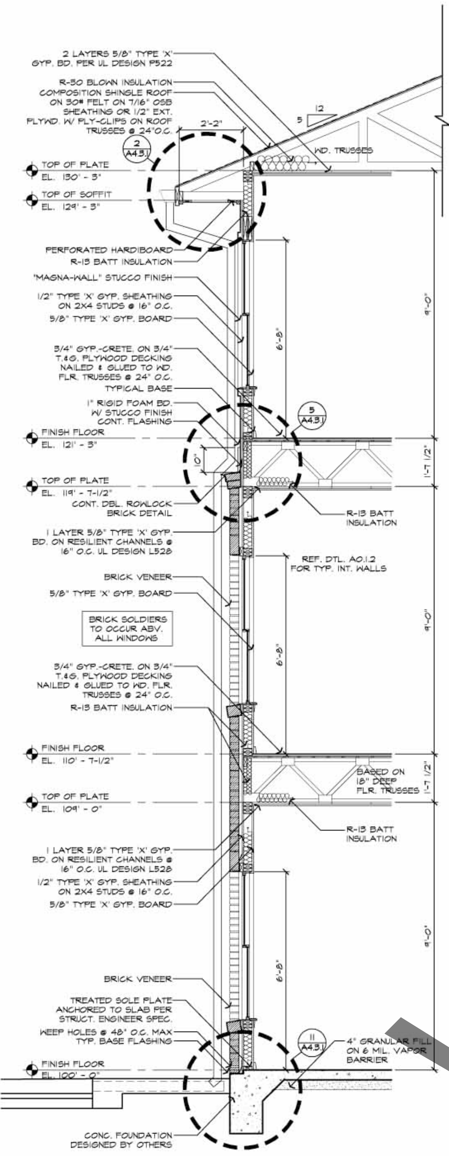
① TYP. WALL SECTION @ WINDOWS 1/2" = 1' - 0" (1/A2.1.2) (1/A2.1.4) (1/A2.2.2) (1/A2.2.4) (1/A2.3.2) (1/A2.3.4) (1/A2.4.2) (1/A2.4.4)
