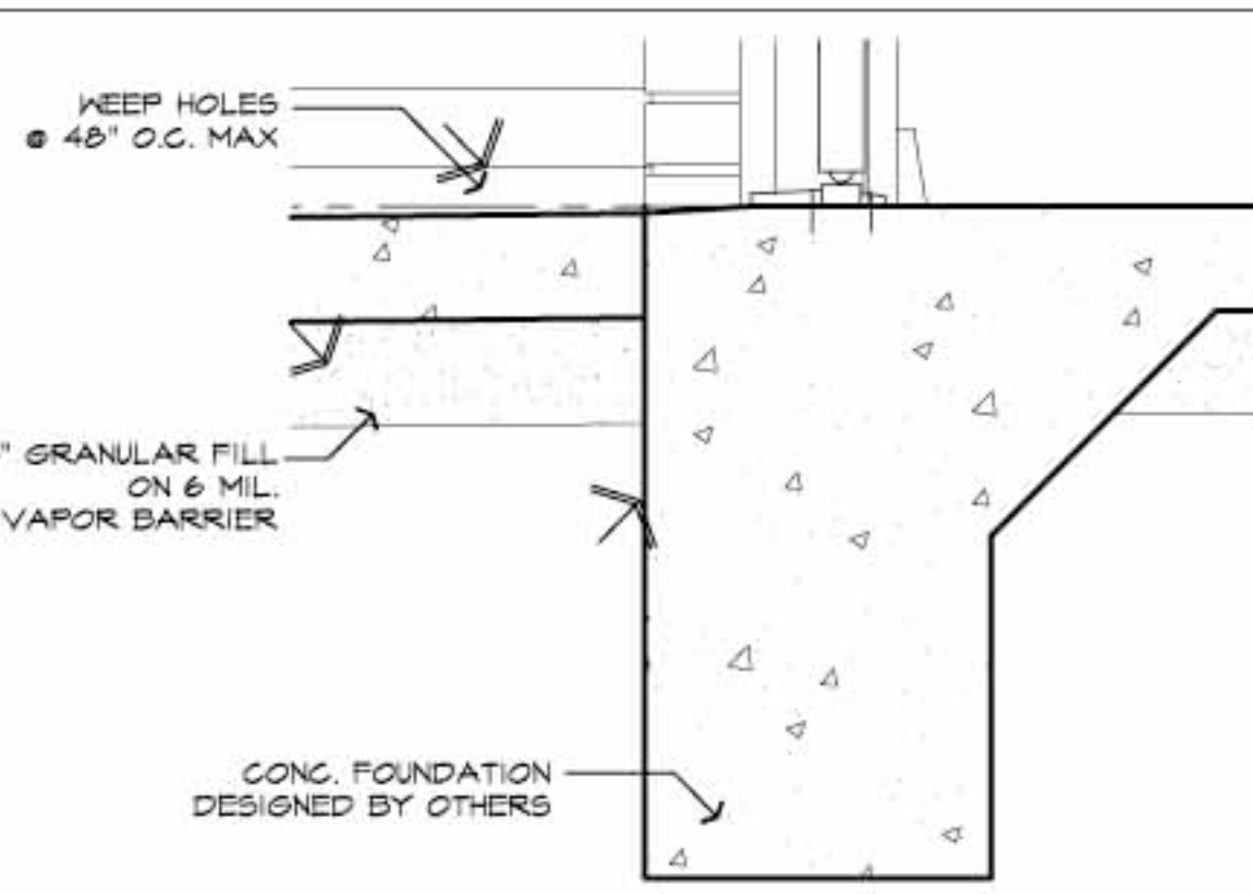
SECTION DETAIL
