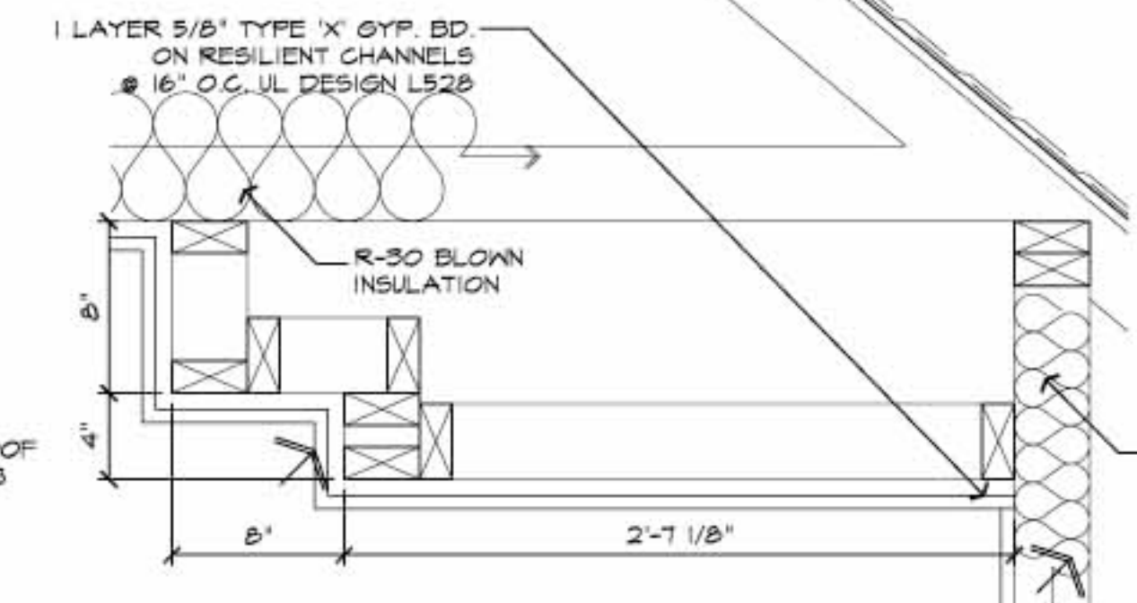
SECTION DETAIL
