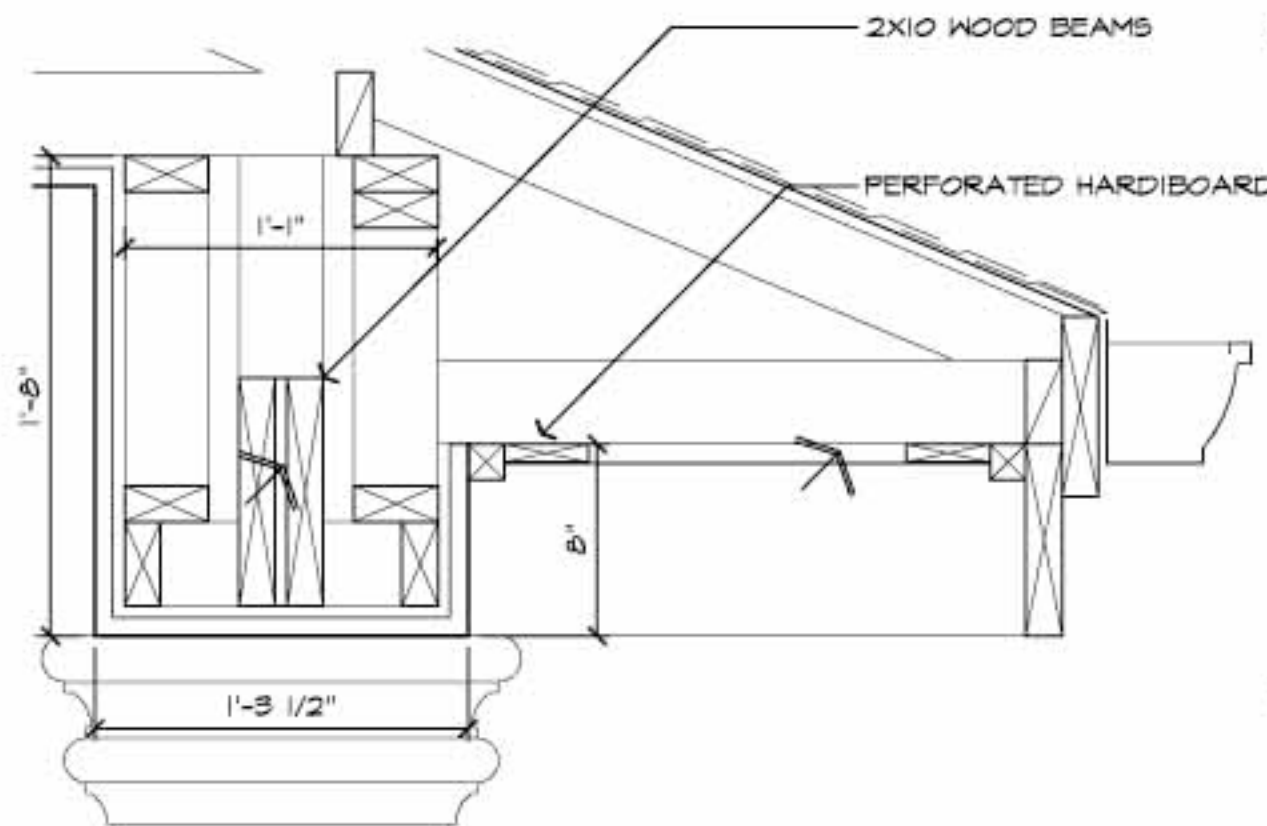
SECTION DETAIL
