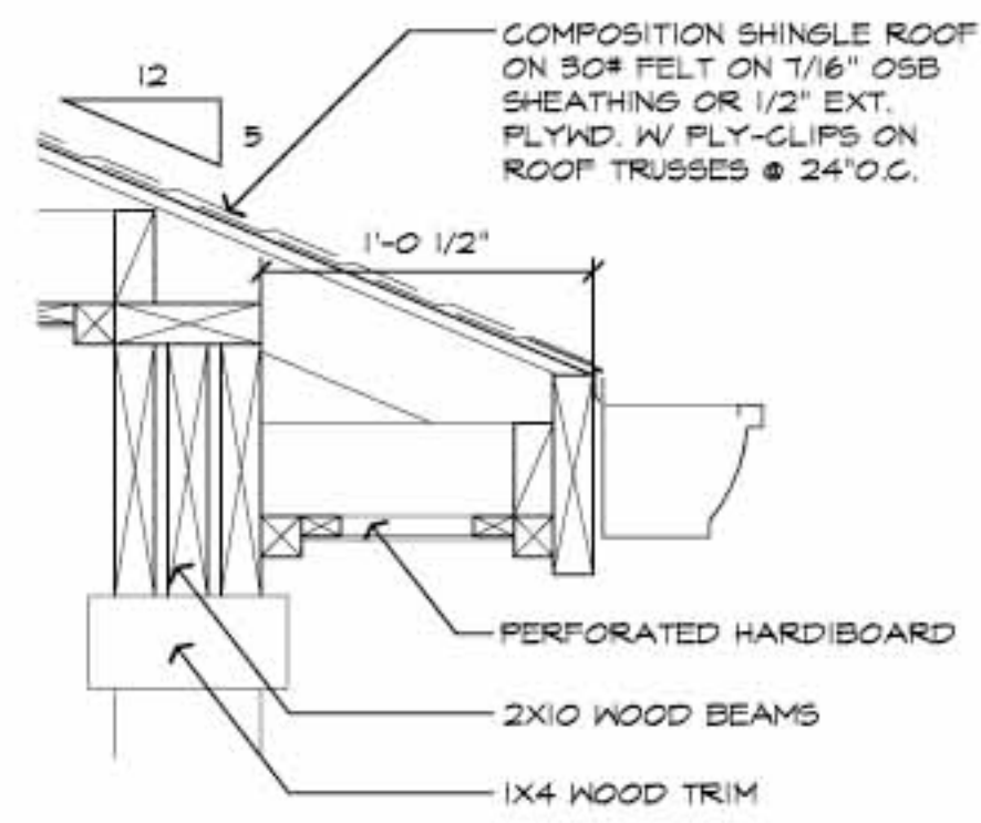
SECTION DETAIL @ WALKWAY
