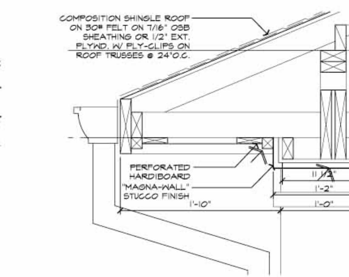
SECTION DETAIL
