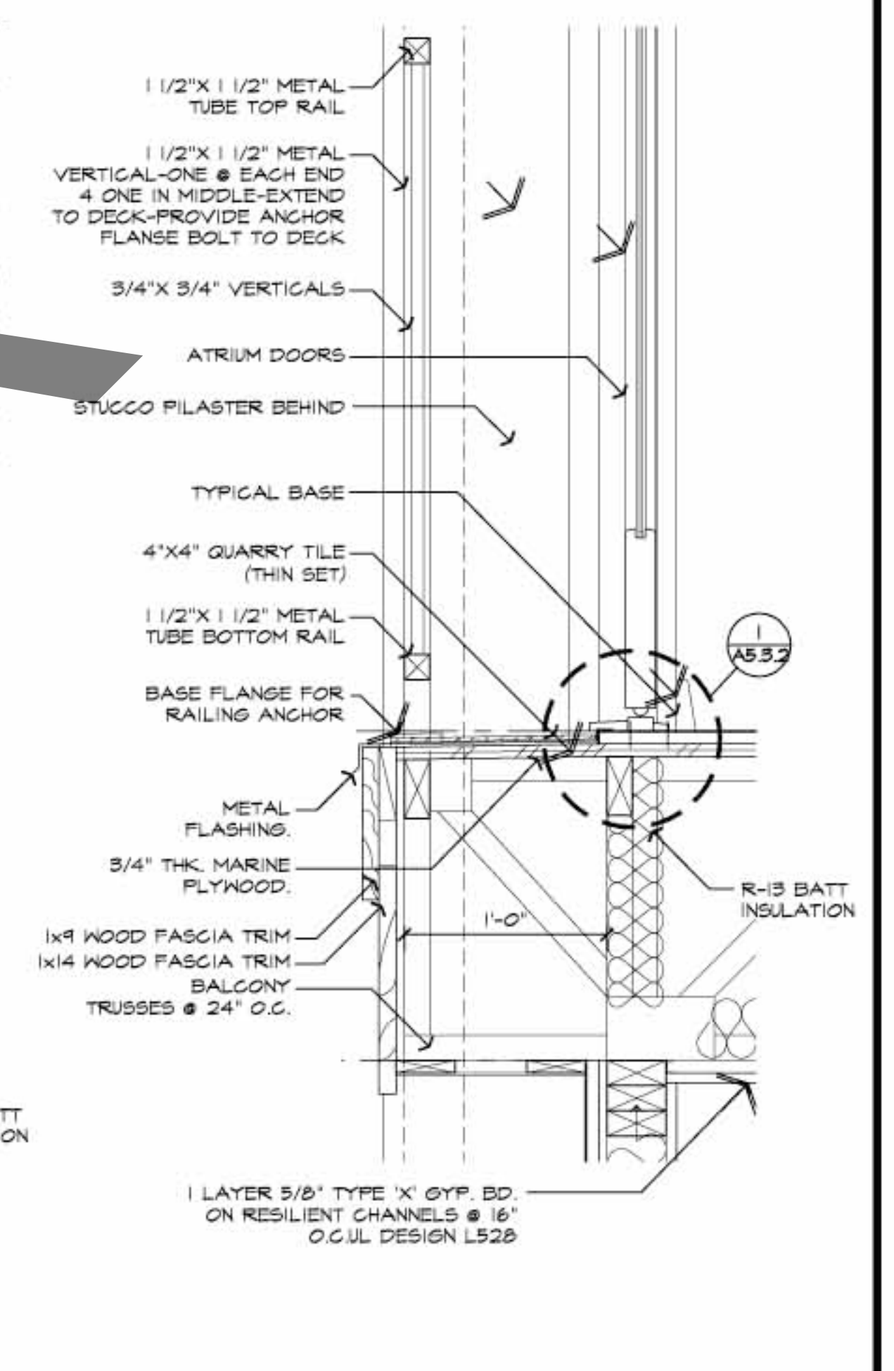
SECTION DETAIL
