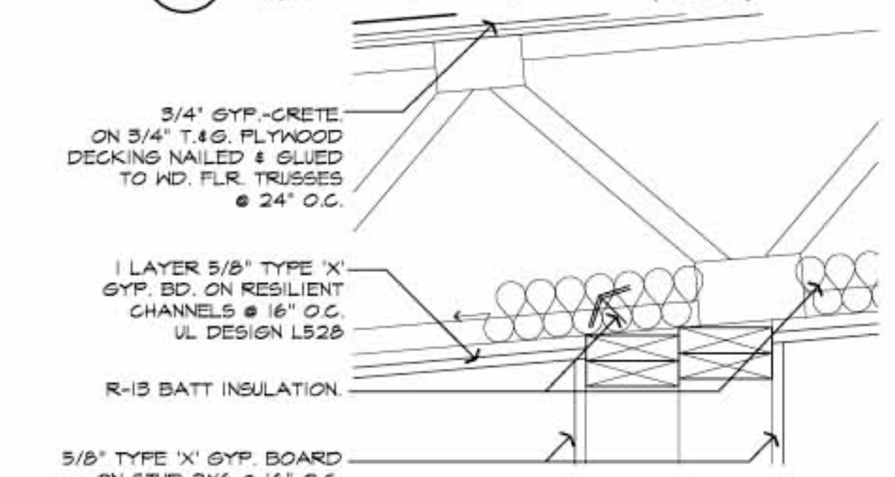
SECTION DETAIL
