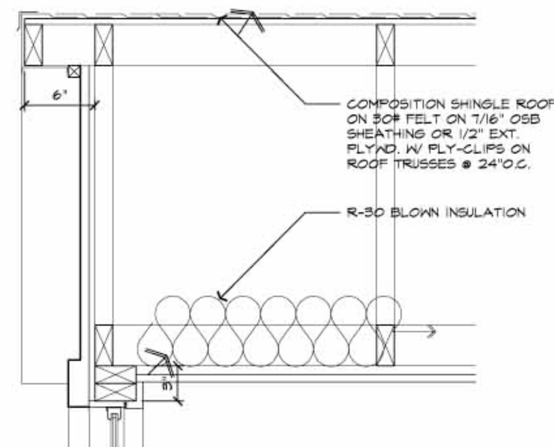
SECTION DETAIL
