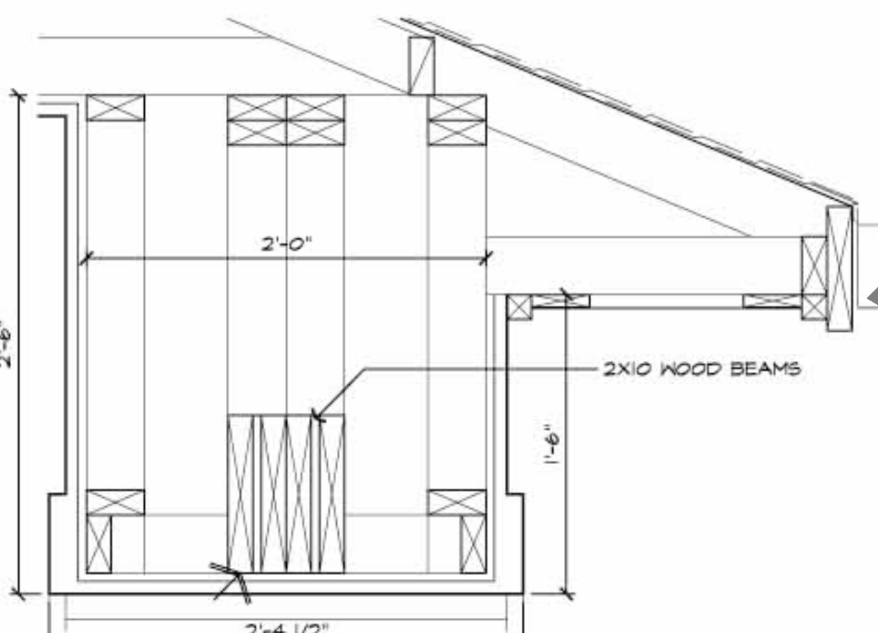
SECTION DETAIL
